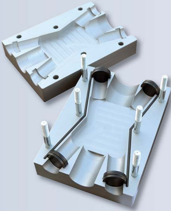
103-10352 X-Block used to blow the second and third cable in a duct with one existing cable.
