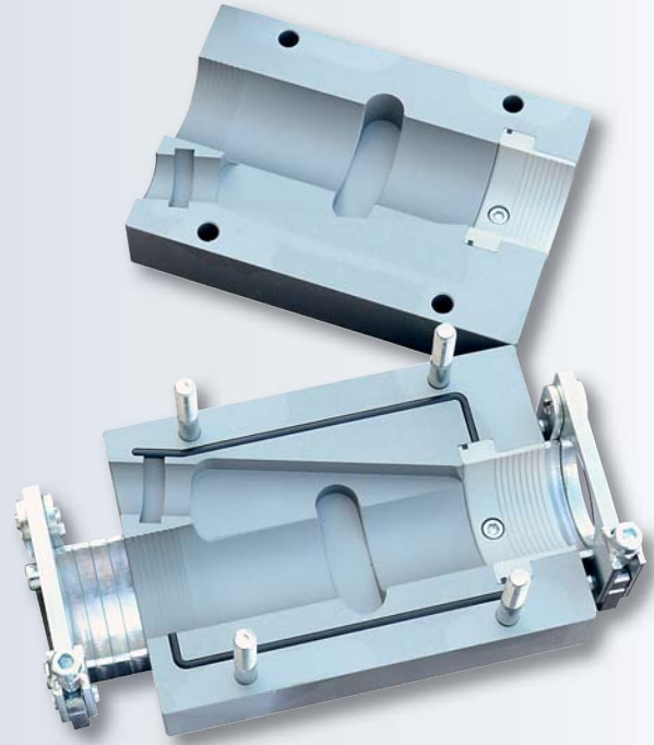
103-10378 Y-Block used to blow the second cable in a duct with one existing cable.
